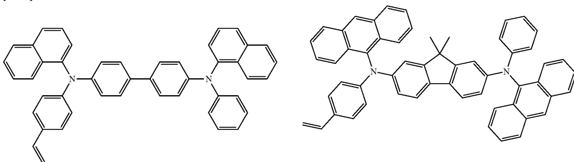
Example of the Polymerizable Monomer (2) [0132]
